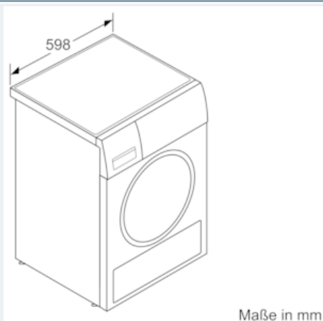
dimensional drawings
