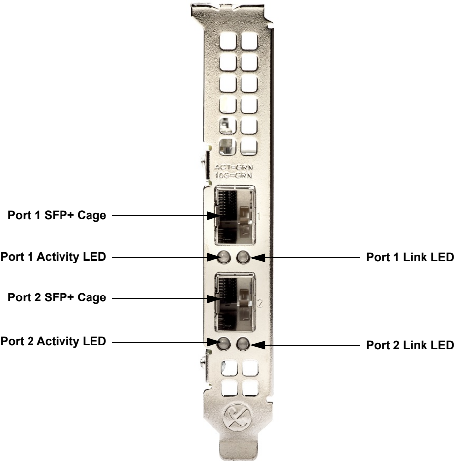
Figure 3: Activity and Link LED Locations
