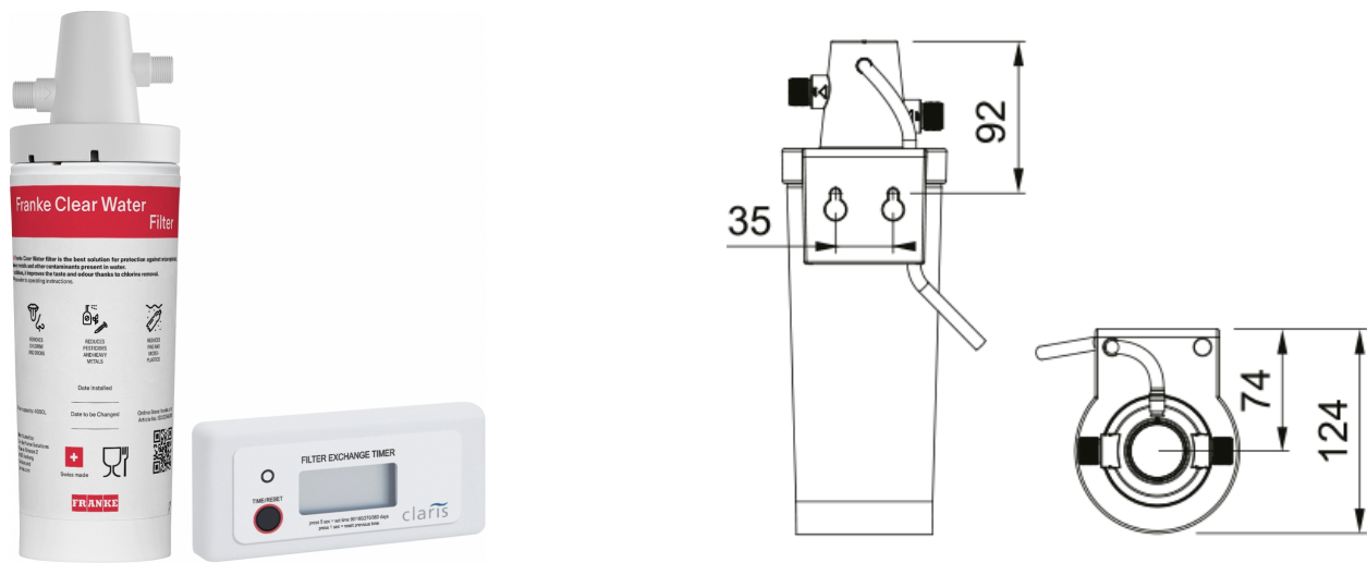
Accessory Clear Water M Filtration set, filter head, filter cartridge, timer
