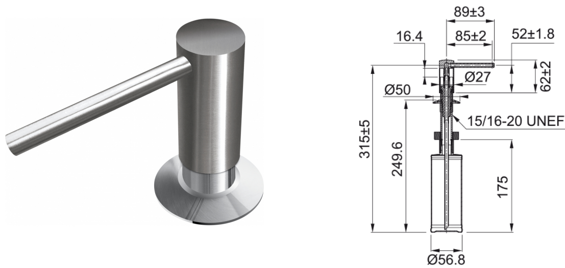
Soap dispenser Comfort SS Optics
