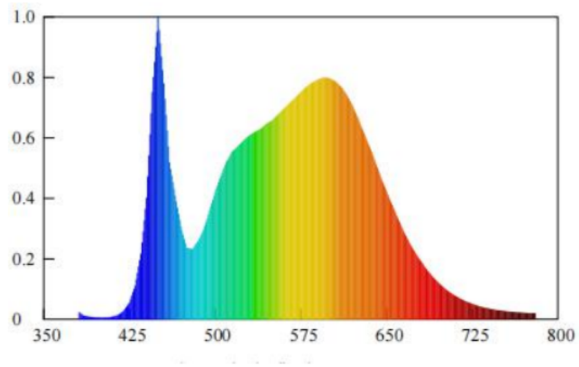
Spectral power distribution at 4000K
