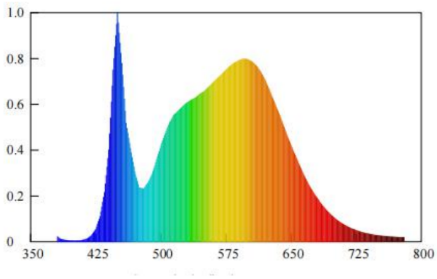
Spectral power distribution at 4000K
