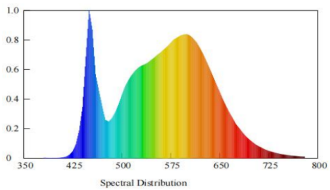
Spectral power distribution at 4000K
