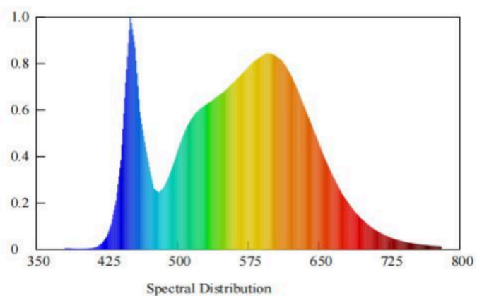
Spectral power distribution at 4000K
