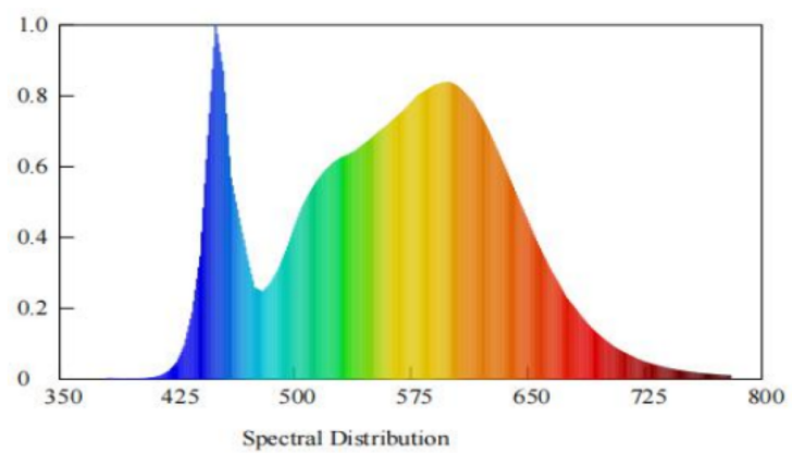
Spectral power distribution at 4000K
