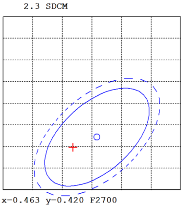
CIE1931 Chromaticity Diagram
