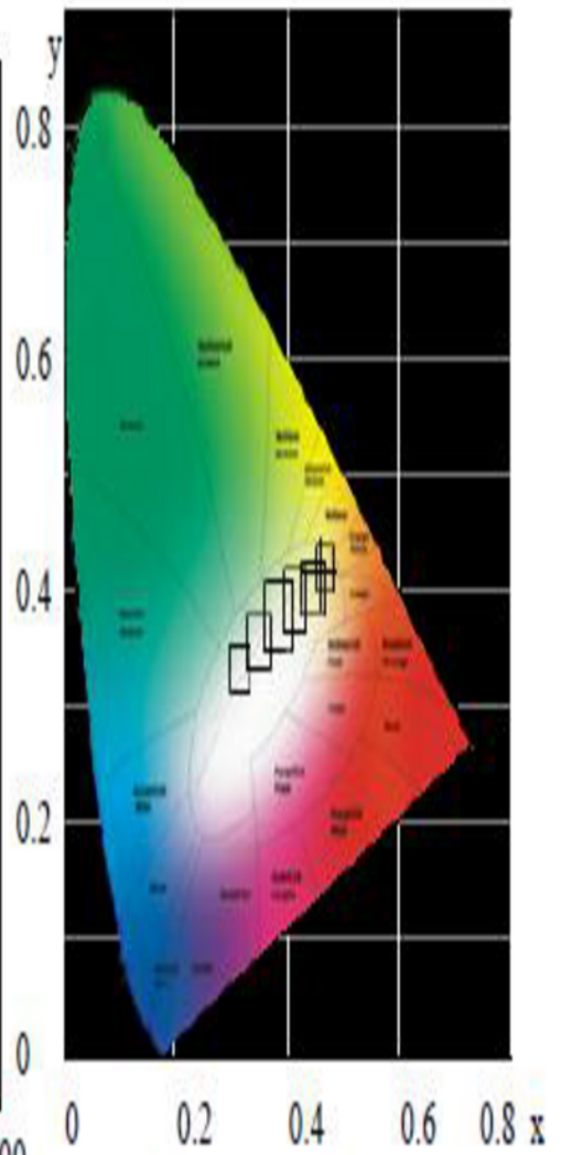
CIE1931 Chromaticity Diagram
