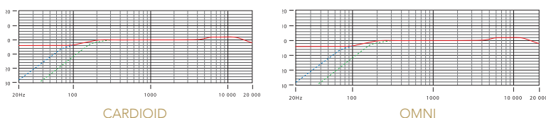
CARDIOID
