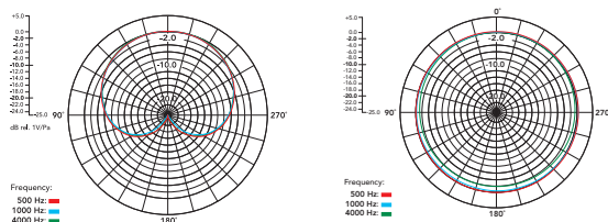
CARDIOID CAPSULE
